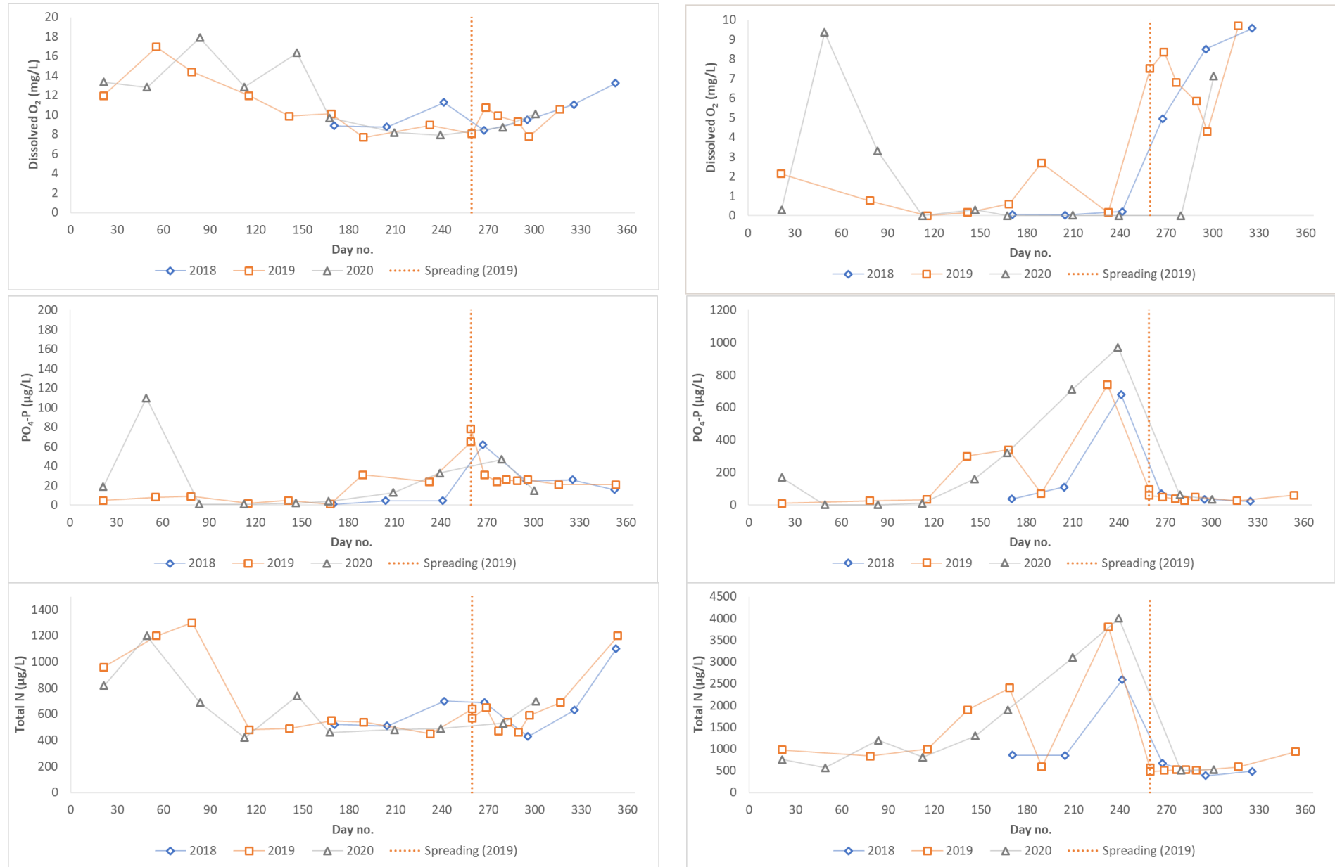
Figure 2.3. Concentrations of dissolved O_2 , PO_4 , and total N in the surface (left) and bottom water (right) in Kyrkviken Bay. Note different scales on the y-axes.
