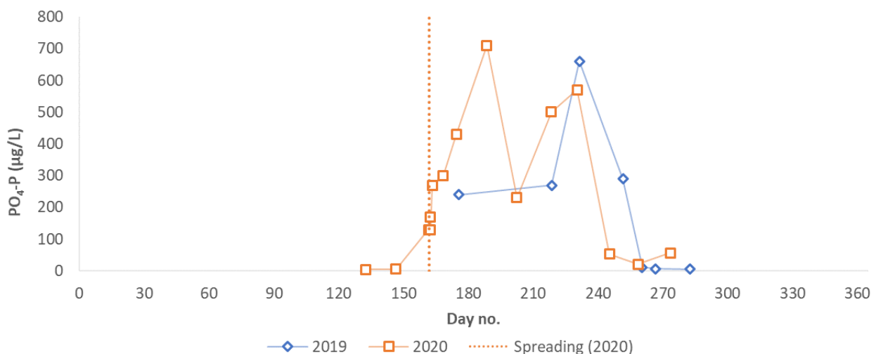
Figure 4.3 Dissolved PO 4 concentration in the bottom water of Kolkka Bay. Dashed line indicates the spreading of marls sorbent in June 2020.
